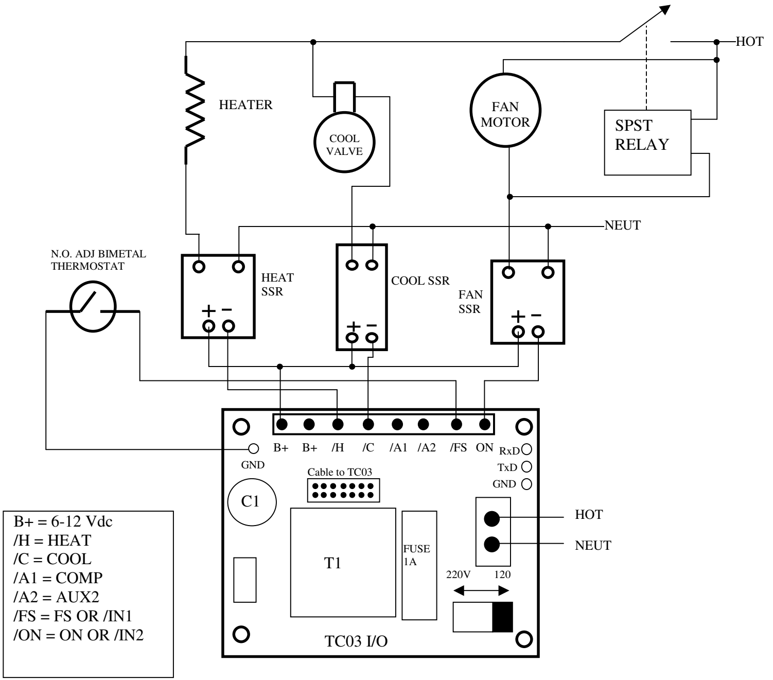
Example hookup of TC03 I/O board
